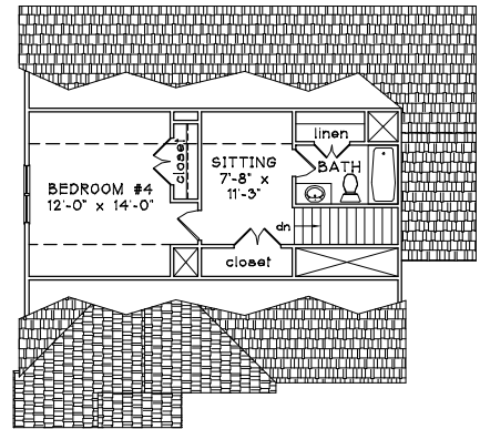
ATTIC PLAN
